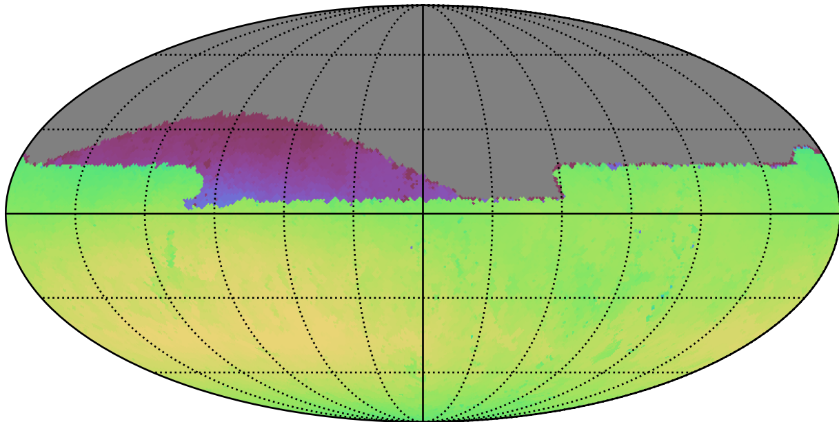
baseline_v3.3_10yrs Yr 1 all bands: Max skyBrightness
