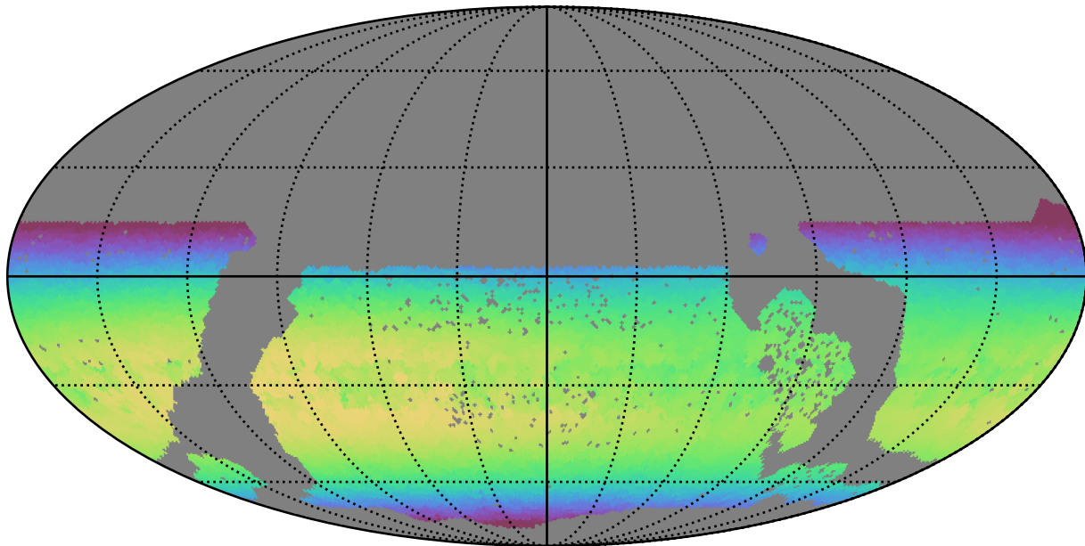
baseline_v3.3_10yrs WFD z band: Max skyBrightness
