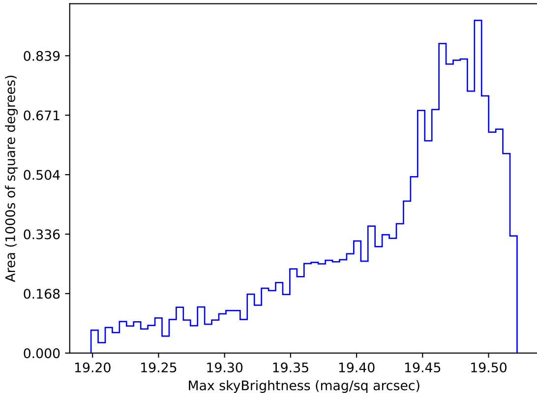
baseline_v3.3_10yrs WFD z band: Max skyBrightness
