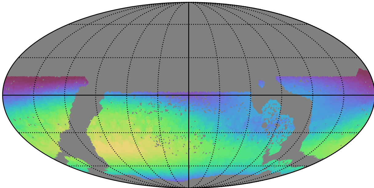
baseline_v3.3_10yrs WFD u band: Max skyBrightness
