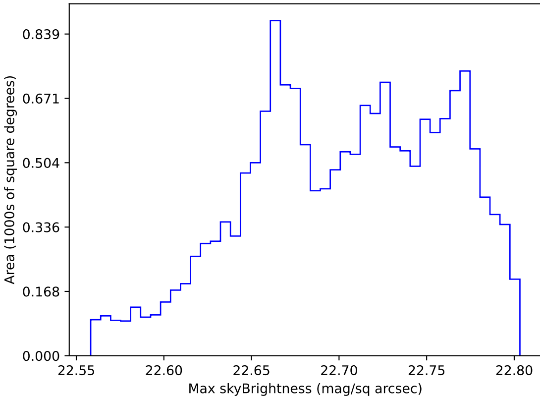
baseline_v3.3_10yrs WFD u band: Max skyBrightness
