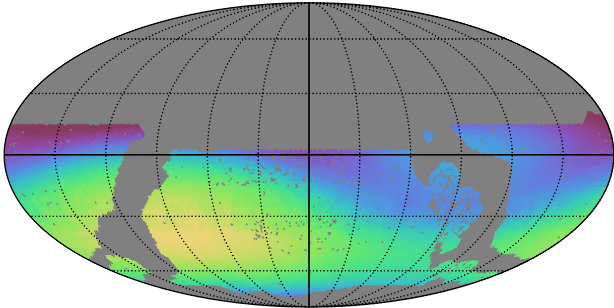
baseline_v3.3_10yrs WFD r band: Max skyBrightness
