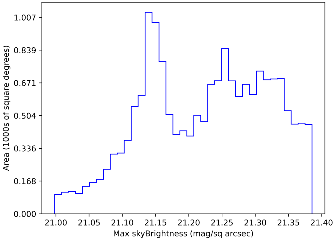
baseline_v3.3_10yrs WFD r band: Max skyBrightness
