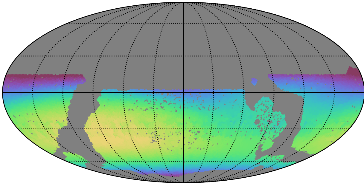
baseline_v3.3_10yrs WFD i band: Max skyBrightness
