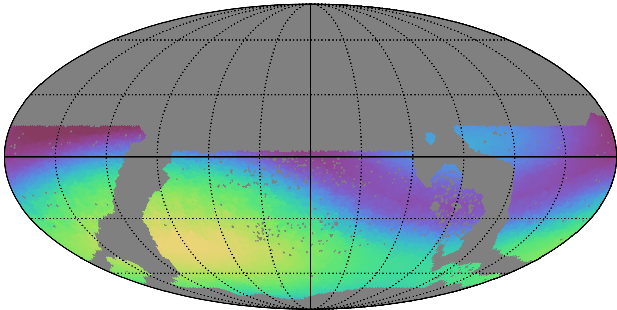
baseline_v3.3_10yrs WFD g band: Max skyBrightness
