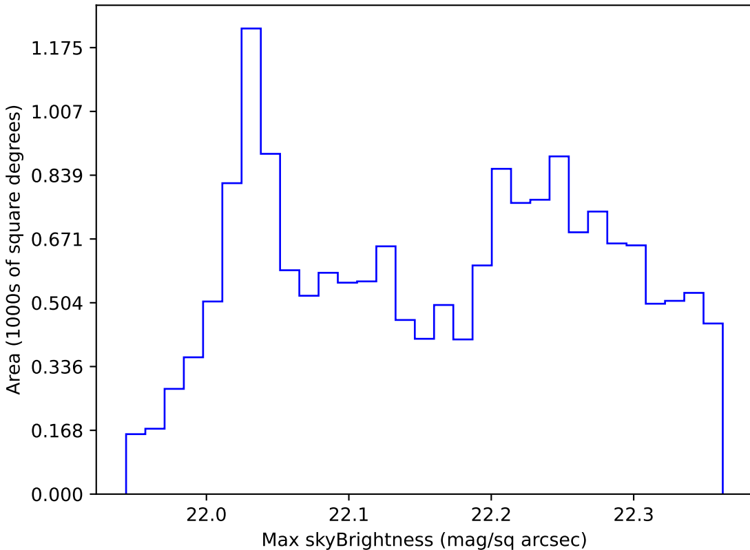
baseline_v3.3_10yrs WFD g band: Max skyBrightness
