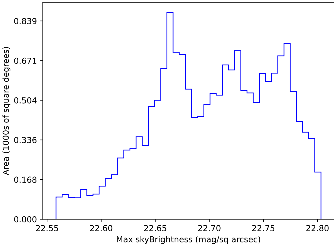
baseline_v3.3_10yrs WFD all bands: Max skyBrightness
