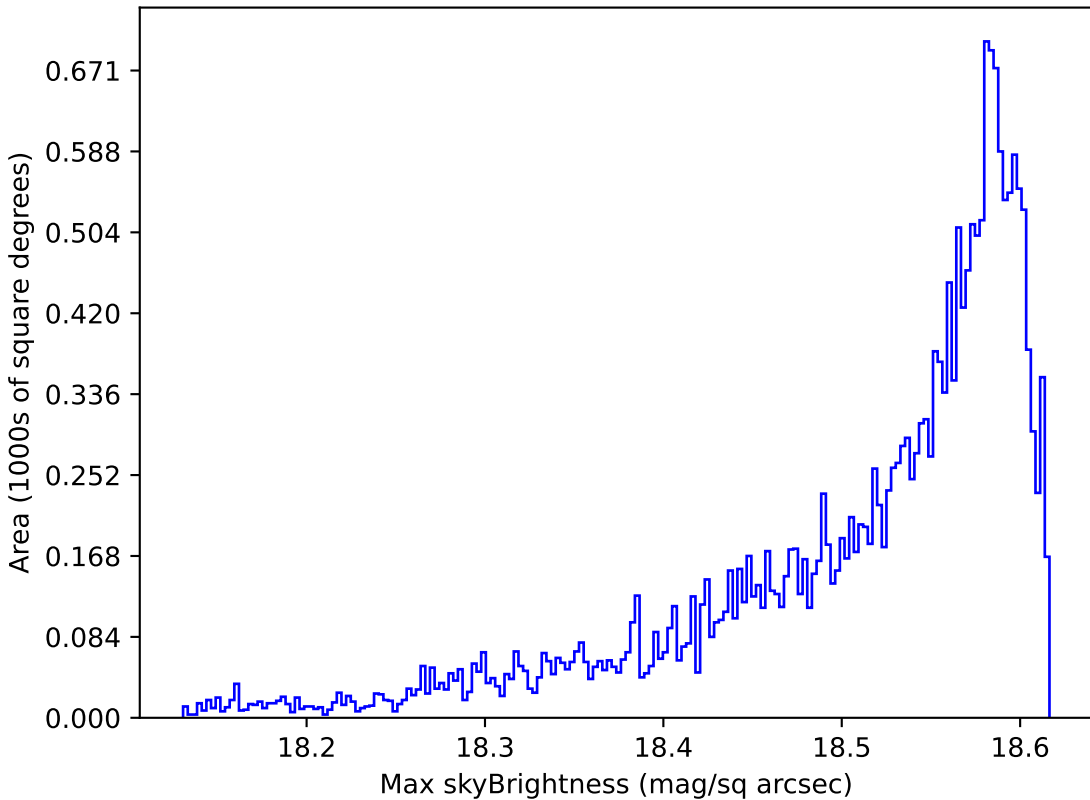
baseline_v3.3_10yrs All sky y band: Max skyBrightness
