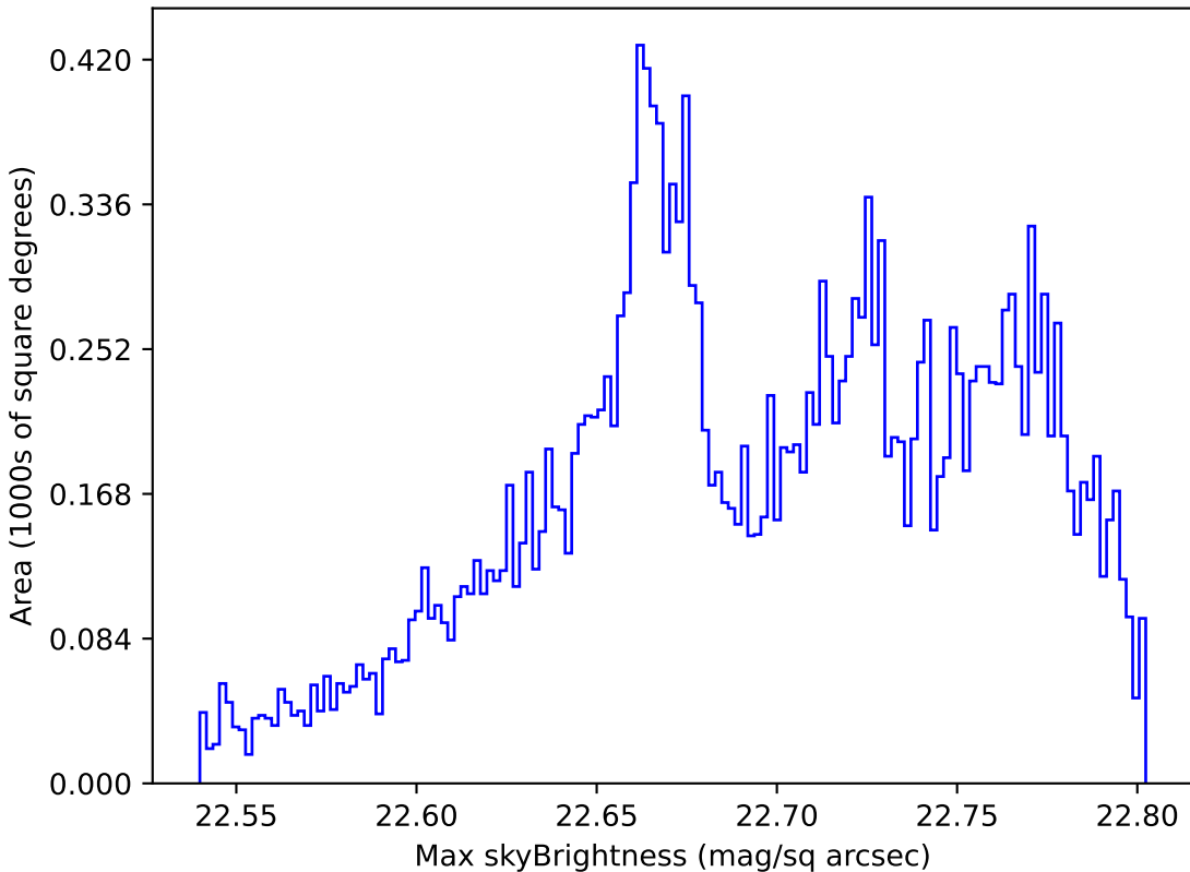
baseline_v3.3_10yrs All sky u band: Max skyBrightness
