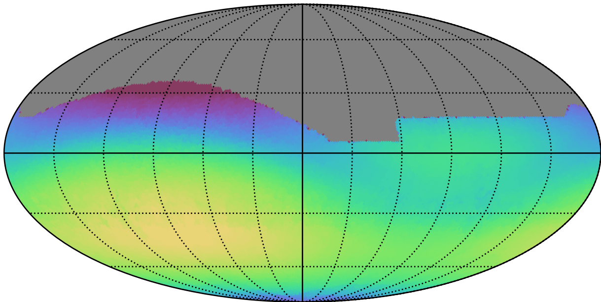
baseline_v3.3_10yrs All sky r band: Max skyBrightness
