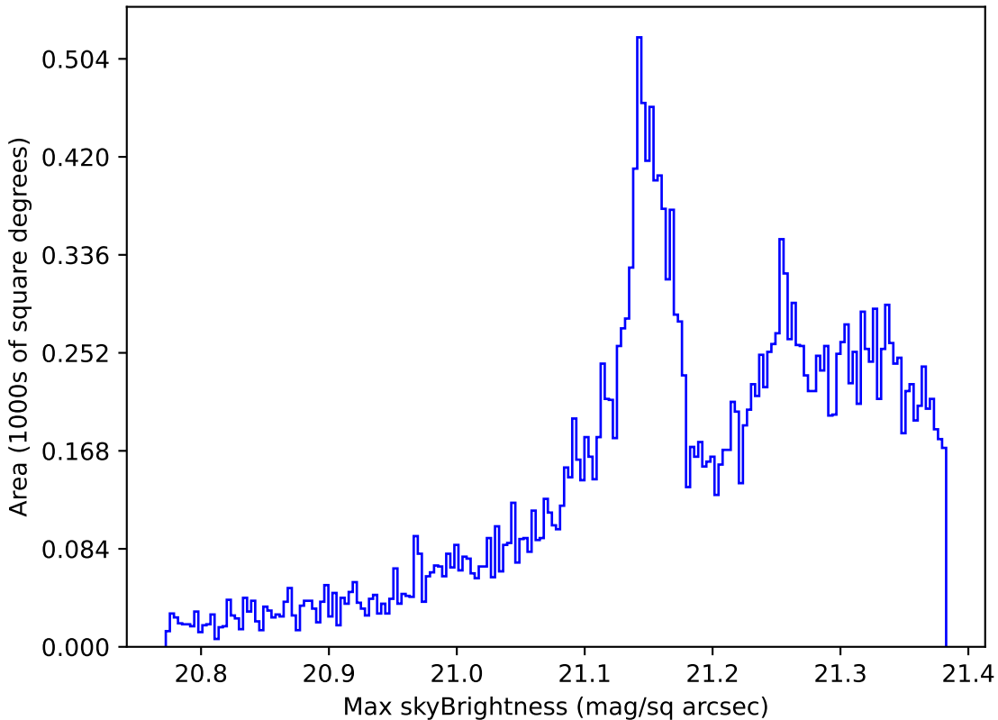
baseline_v3.3_10yrs All sky r band: Max skyBrightness
