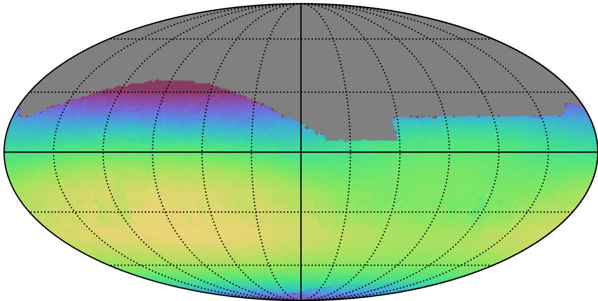
baseline_v3.3_10yrs All sky i band: Max skyBrightness
