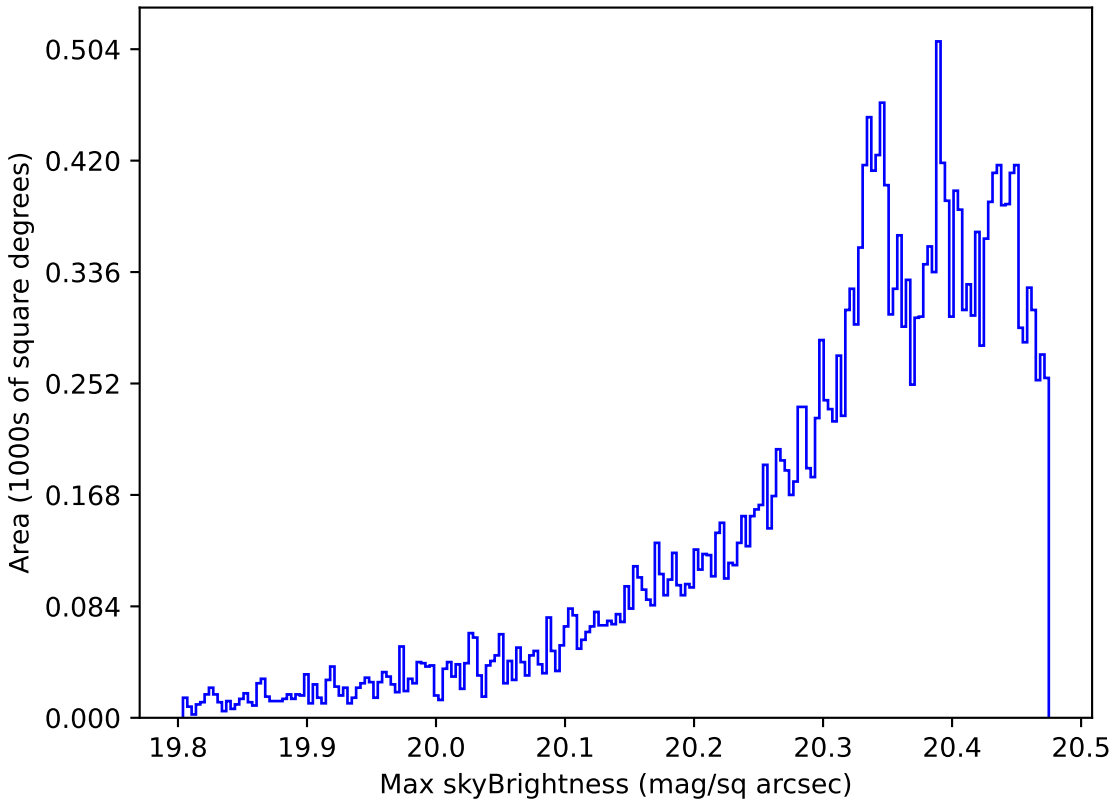
baseline_v3.3_10yrs All sky i band: Max skyBrightness
