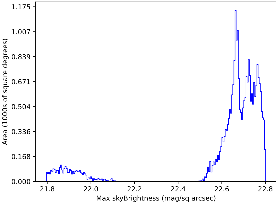
baseline_v3.3_10yrs All sky all bands: Max skyBrightness
