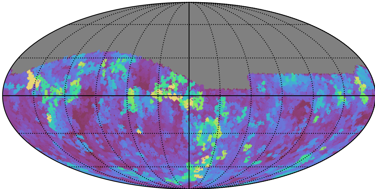
baseline_v3.3_10yrs Yr 1 z band: Max seeingGeom
