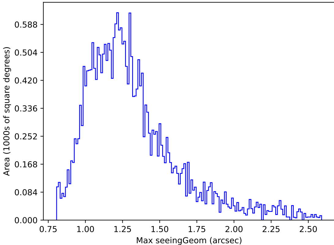
baseline_v3.3_10yrs Yr 1 z band: Max seeingGeom
