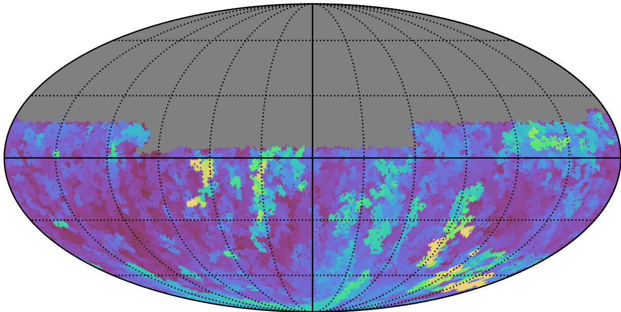
baseline_v3.3_10yrs Yr 1 u band: Max seeingGeom
