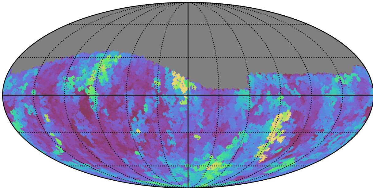
baseline_v3.3_10yrs Yr 1 g band: Max seeingGeom
