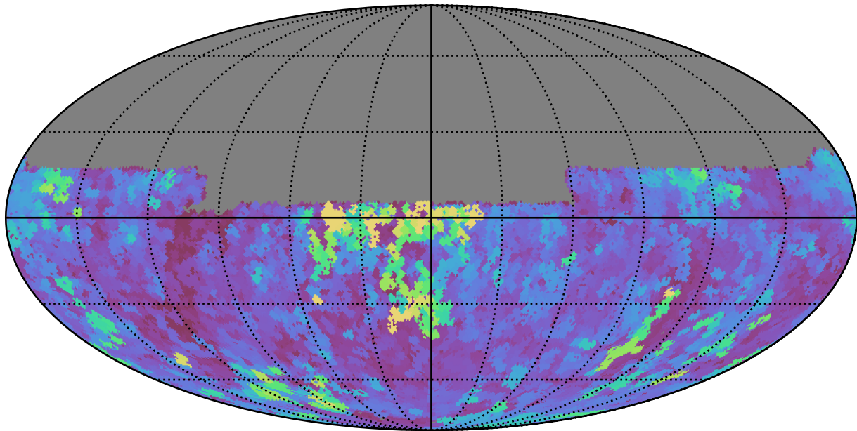
baseline_v3.3_10yrs Yr 1 y band: Max seeingEff
