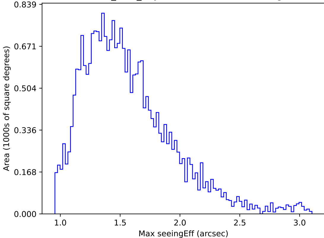
baseline_v3.3_10yrs Yr 1 i band: Max seeingEff
