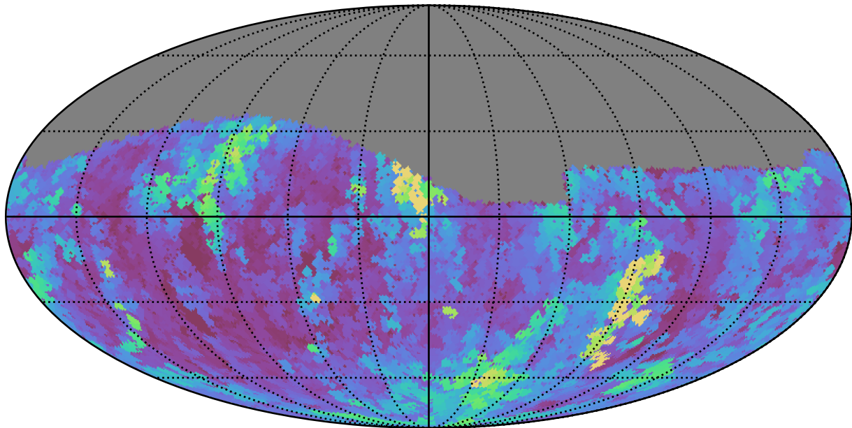
baseline_v3.3_10yrs Yr 1 g band: Max seeingEff
