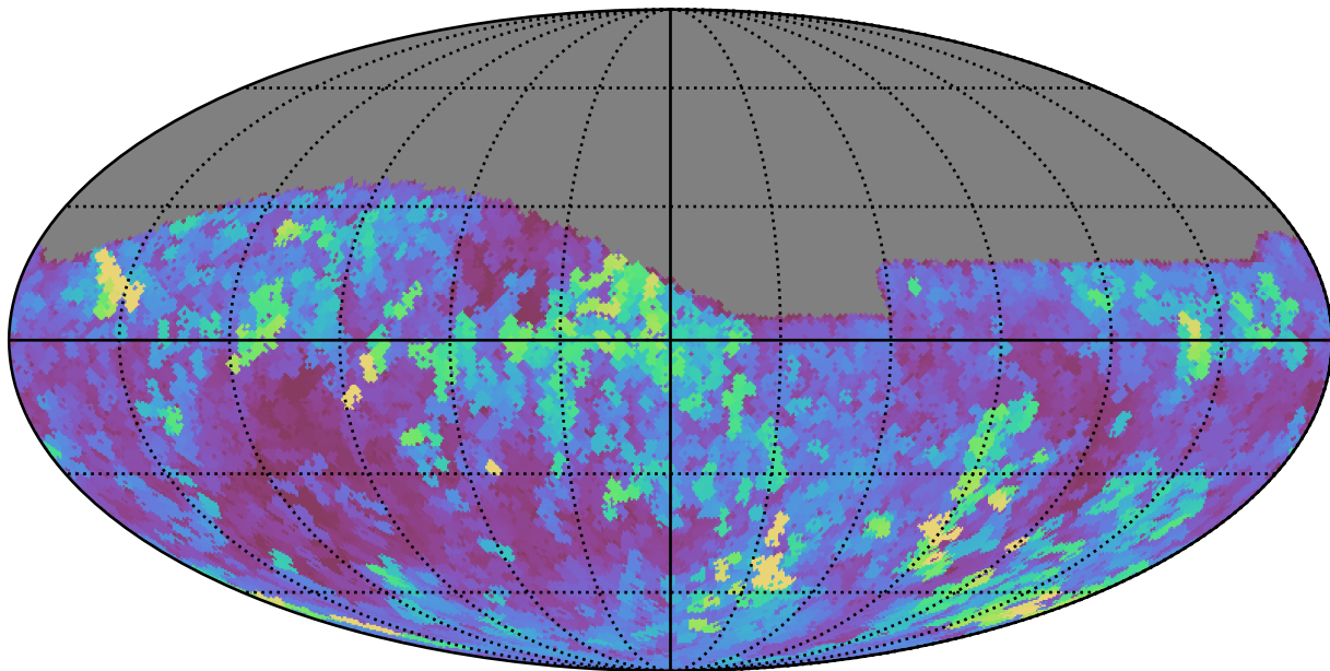
baseline_v3.3_10yrs Yr 1 all bands: Max seeingEff
