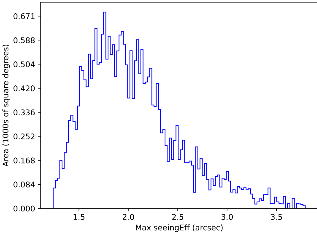
baseline_v3.3_10yrs Yr 1 all bands: Max seeingEff
