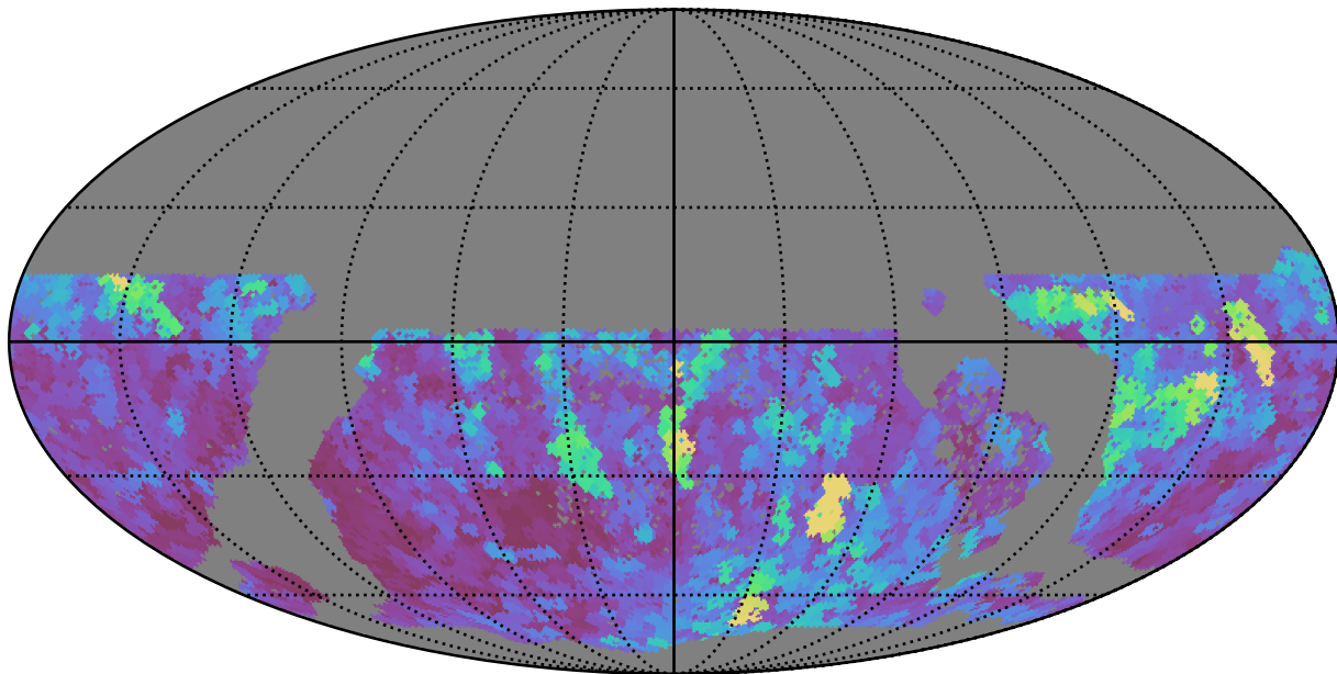
baseline_v3.3_10yrs WFD z band: Max seeingEff
