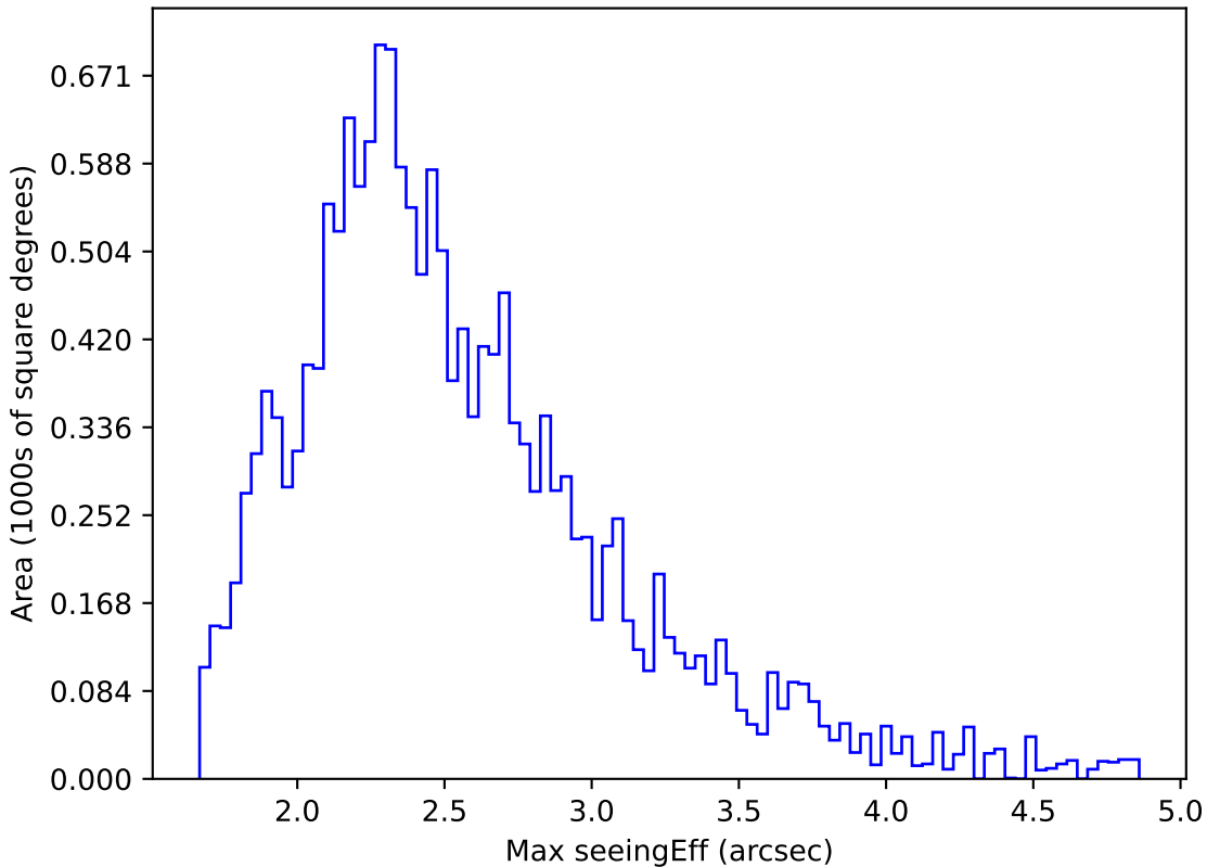
baseline_v3.3_10yrs WFD z band: Max seeingEff
