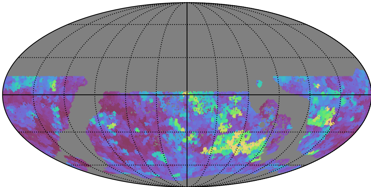
baseline_v3.3_10yrs WFD y band: Max seeingEff
