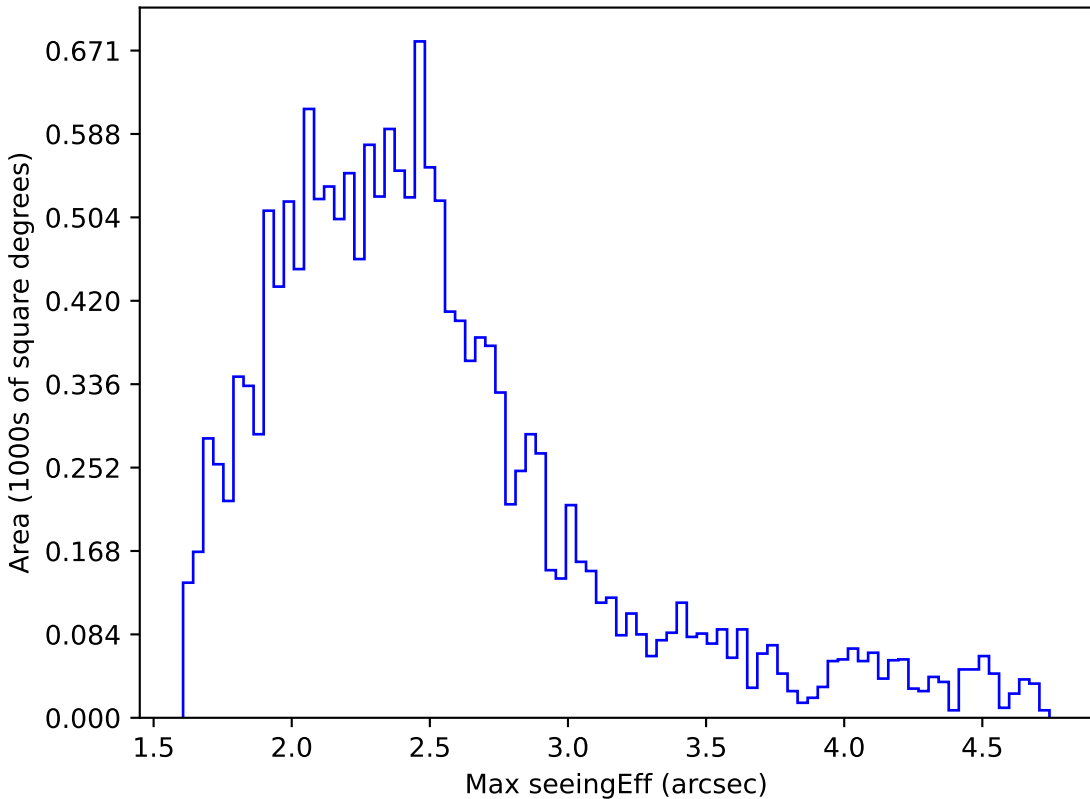
baseline_v3.3_10yrs WFD y band: Max seeingEff
