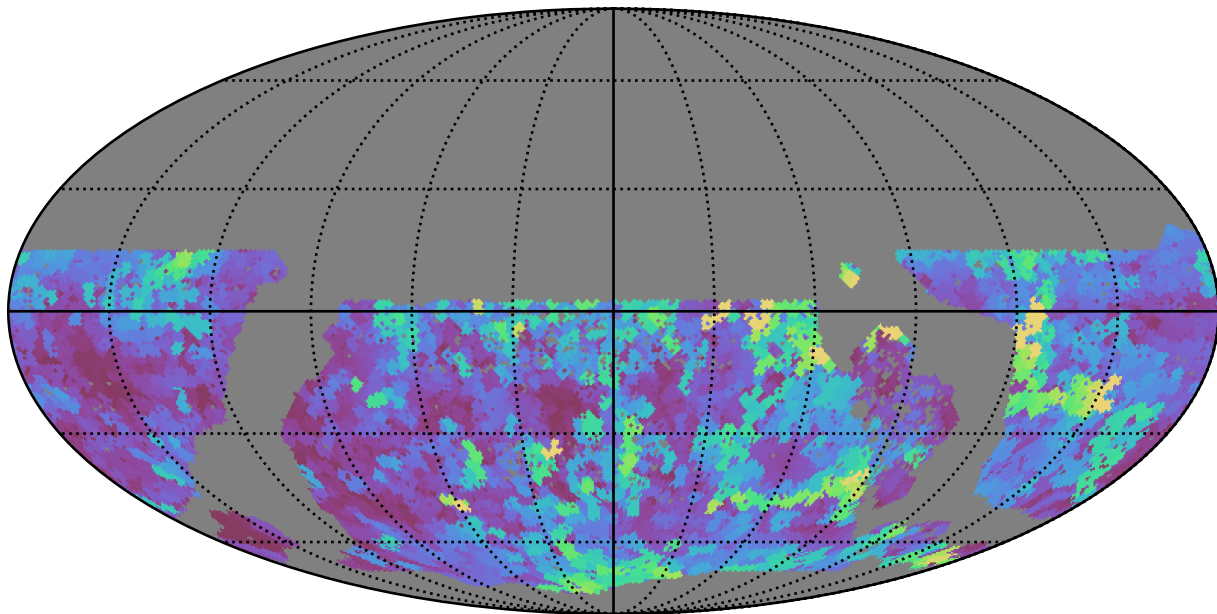
baseline_v3.3_10yrs WFD u band: Max seeingEff
