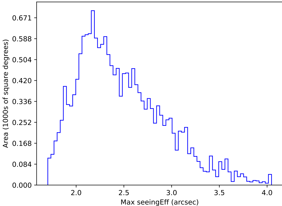
baseline_v3.3_10yrs WFD u band: Max seeingEff
