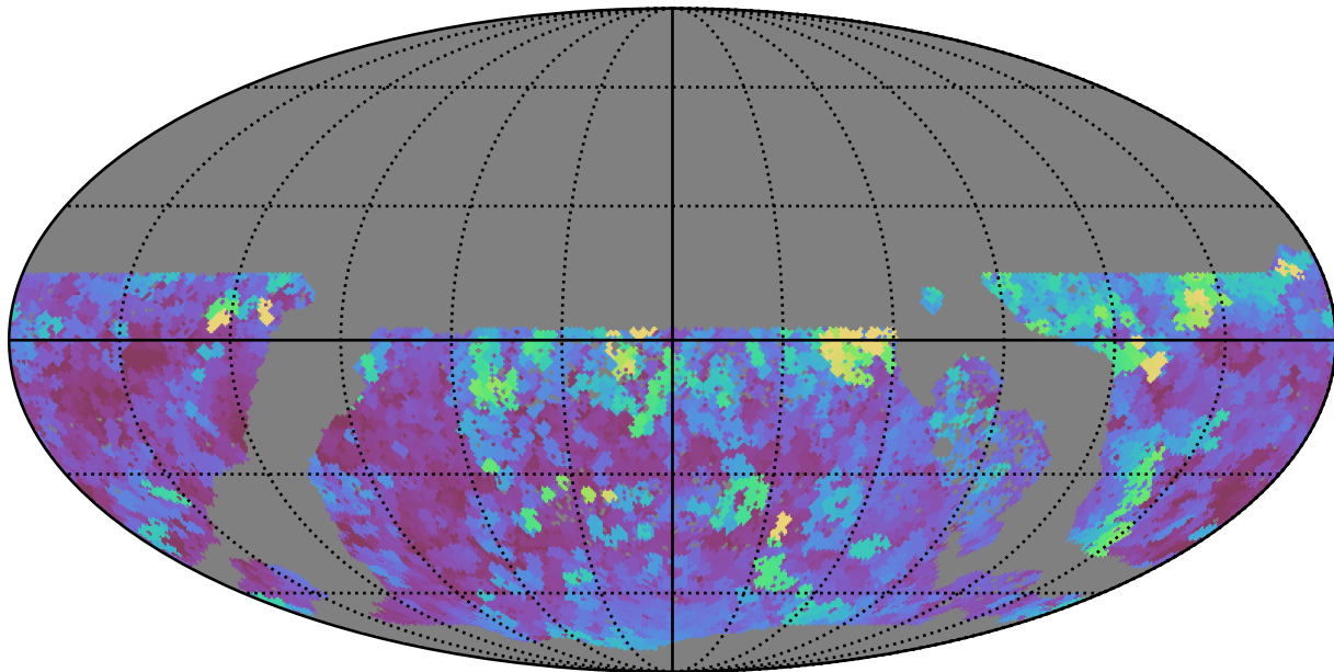
baseline_v3.3_10yrs WFD r band: Max seeingEff
