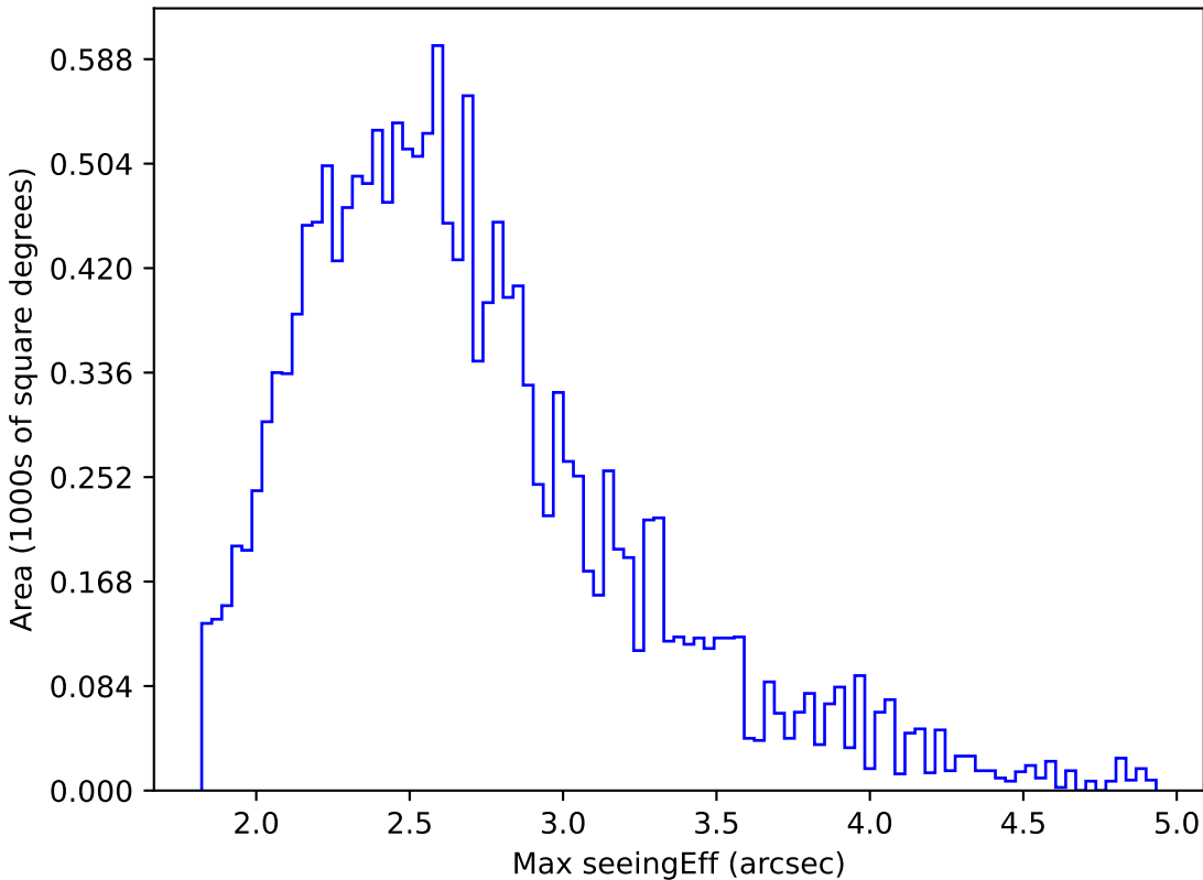
baseline_v3.3_10yrs WFD r band: Max seeingEff
