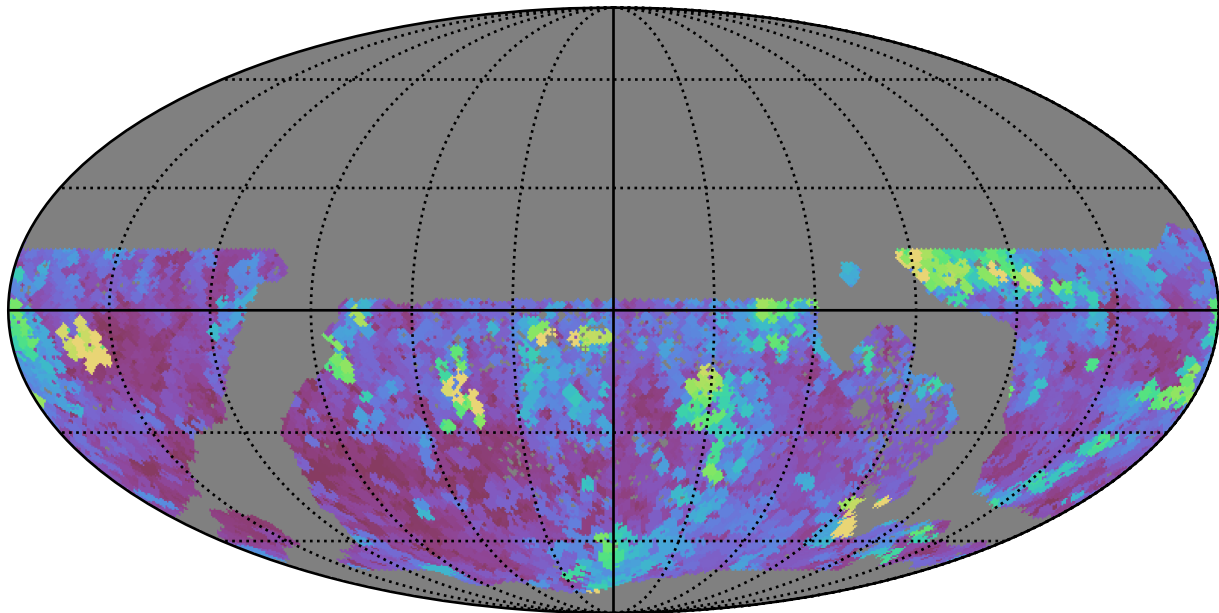
baseline_v3.3_10yrs WFD i band: Max seeingEff
