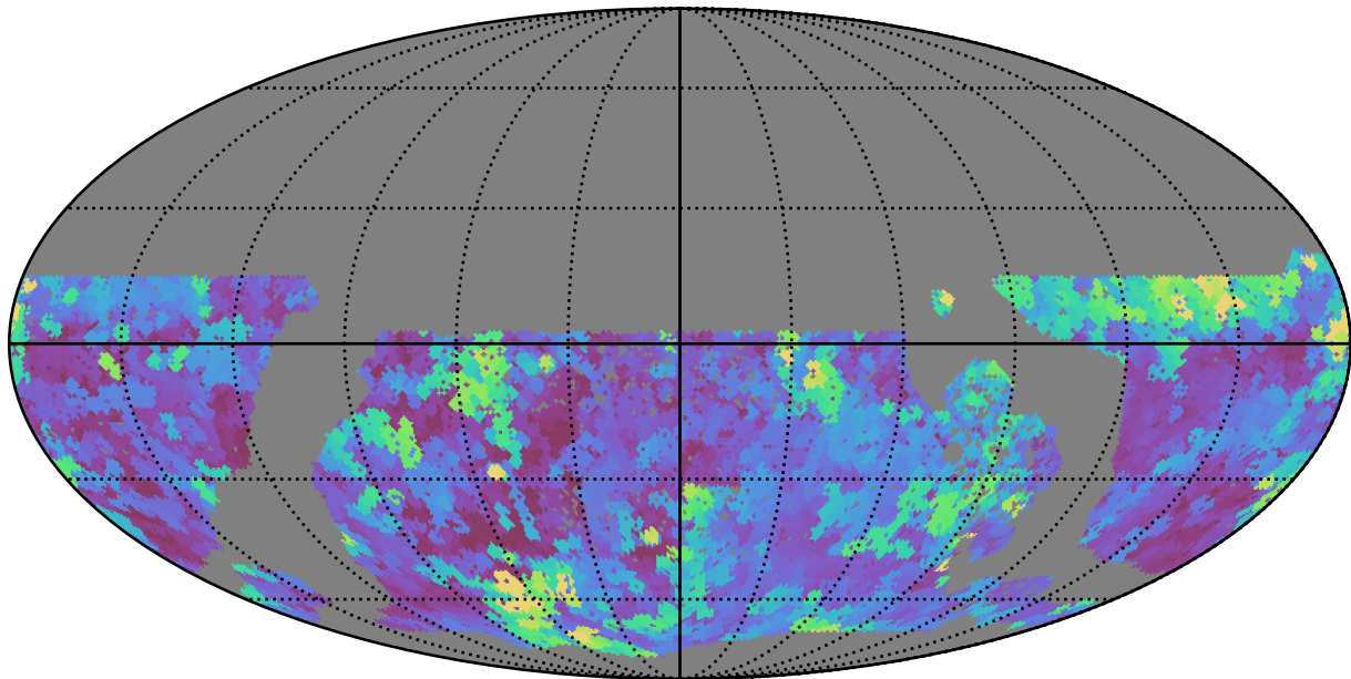
baseline_v3.3_10yrs WFD g band: Max seeingEff
