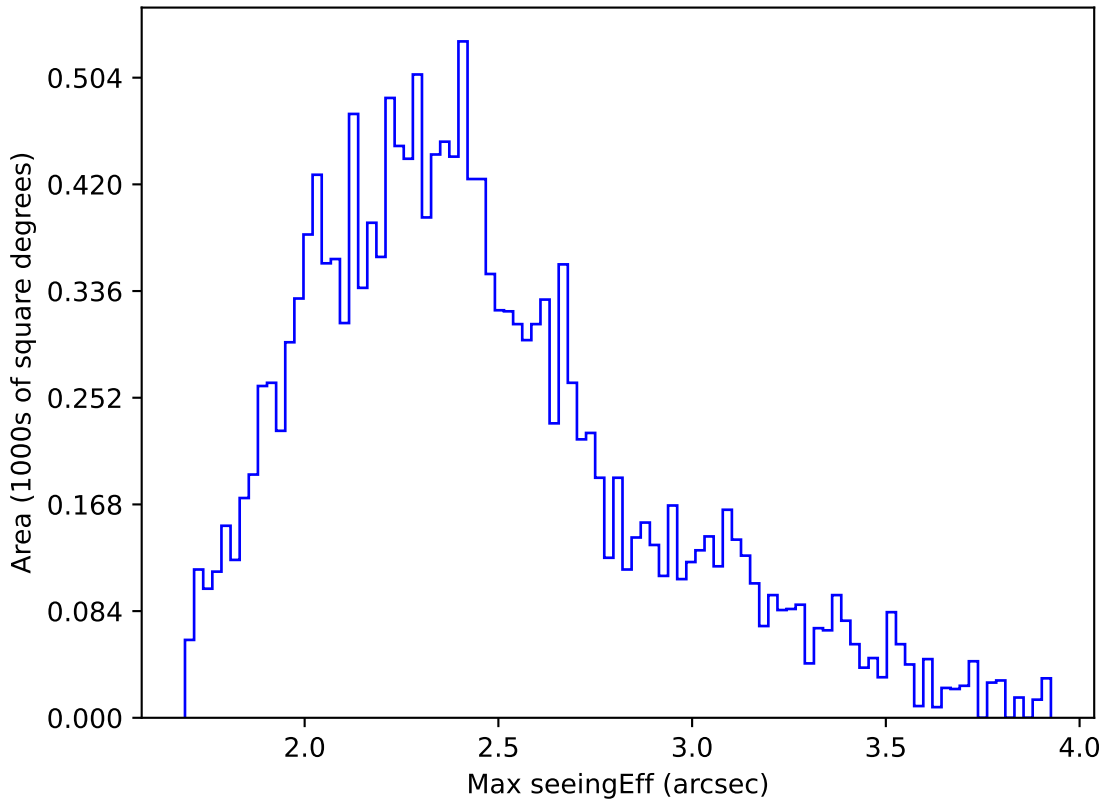
baseline_v3.3_10yrs WFD g band: Max seeingEff
