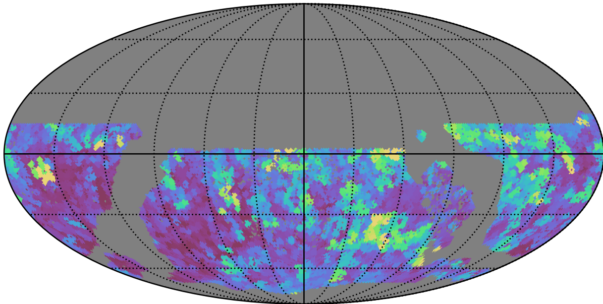
baseline_v3.3_10yrs WFD all bands: Max seeingEff
