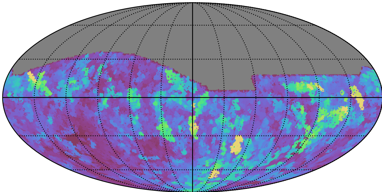
baseline_v3.3_10yrs All sky z band: Max seeingEff
