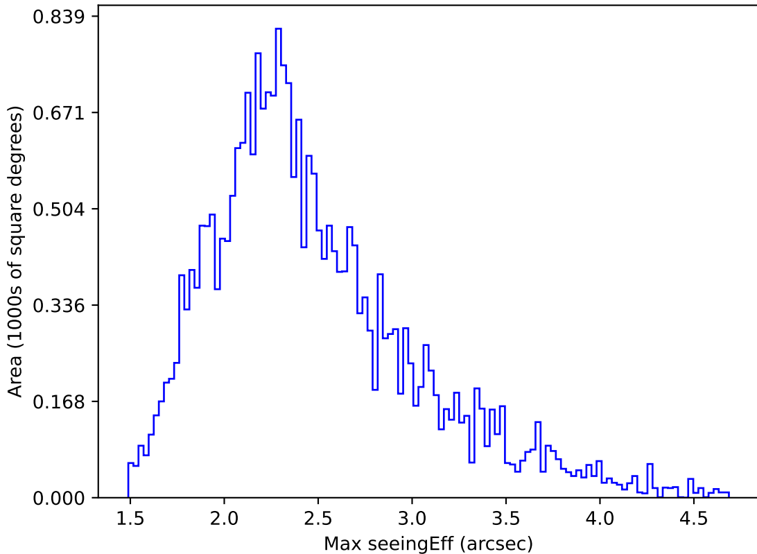
baseline_v3.3_10yrs All sky z band: Max seeingEff
