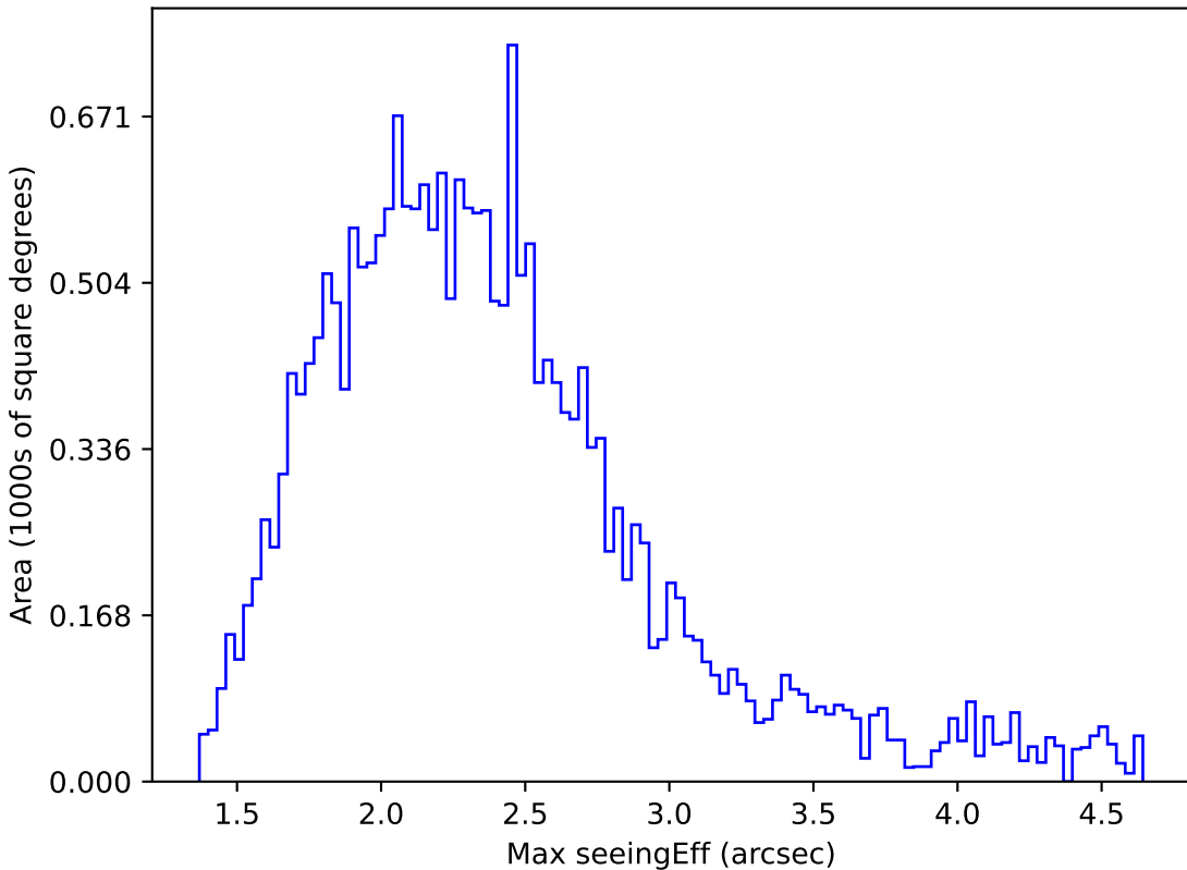
baseline_v3.3_10yrs All sky y band: Max seeingEff
