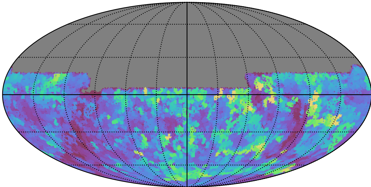
baseline_v3.3_10yrs All sky u band: Max seeingEff
