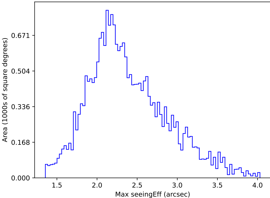
baseline_v3.3_10yrs All sky u band: Max seeingEff
