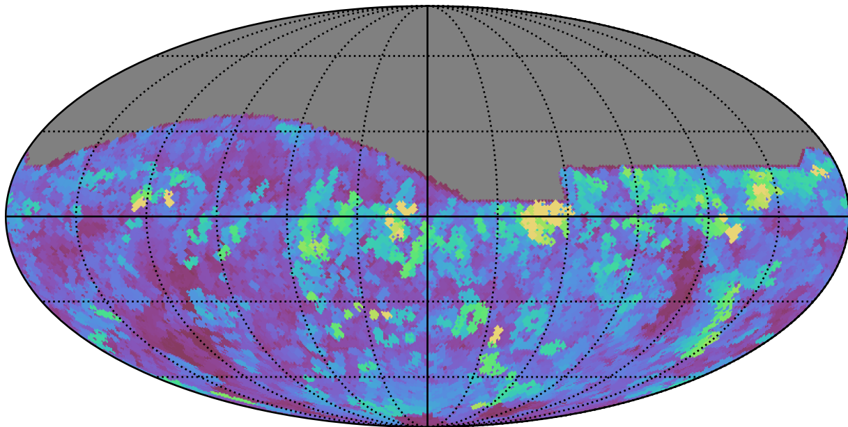
baseline_v3.3_10yrs All sky r band: Max seeingEff
