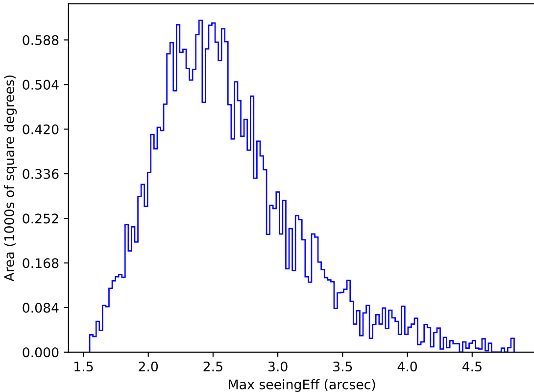
baseline_v3.3_10yrs All sky r band: Max seeingEff
