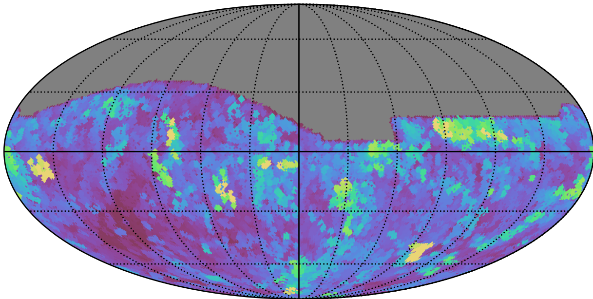
baseline_v3.3_10yrs All sky i band: Max seeingEff
