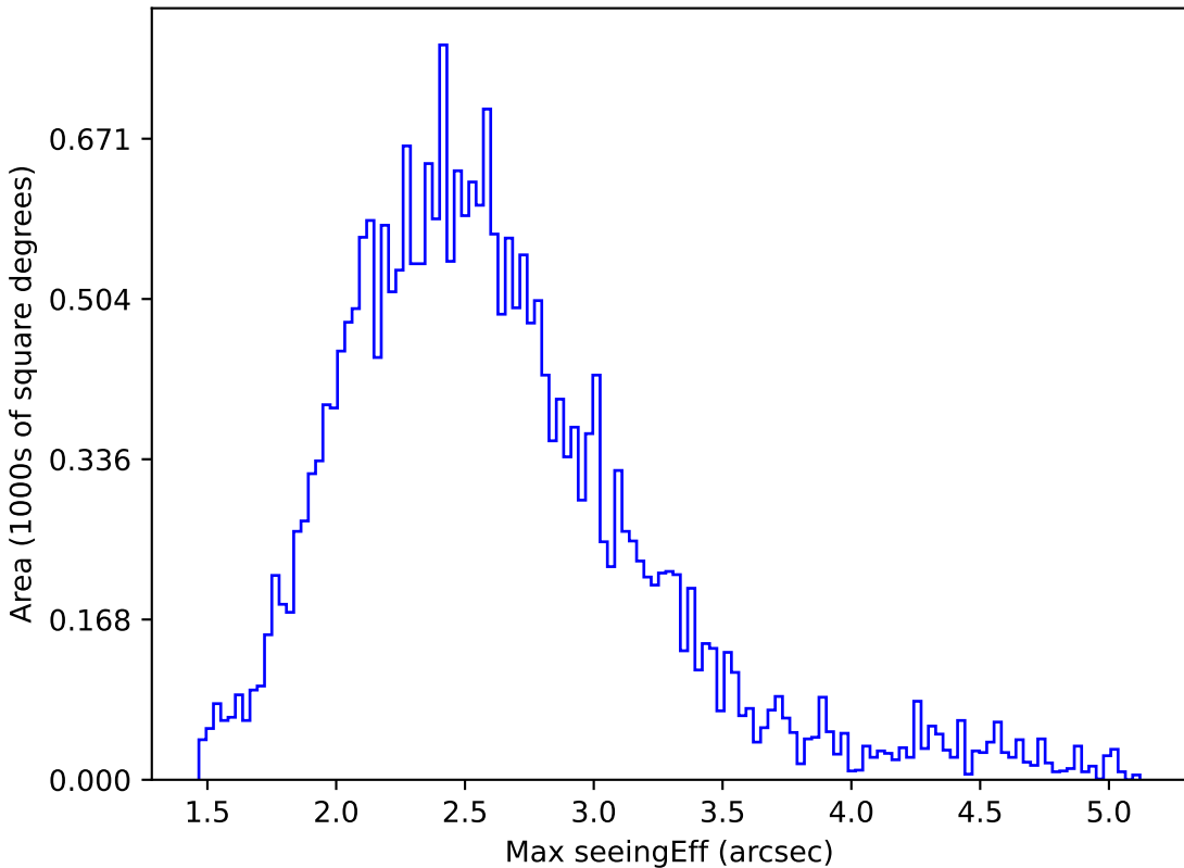
baseline_v3.3_10yrs All sky i band: Max seeingEff
