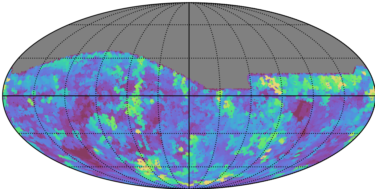
baseline_v3.3_10yrs All sky g band: Max seeingEff
