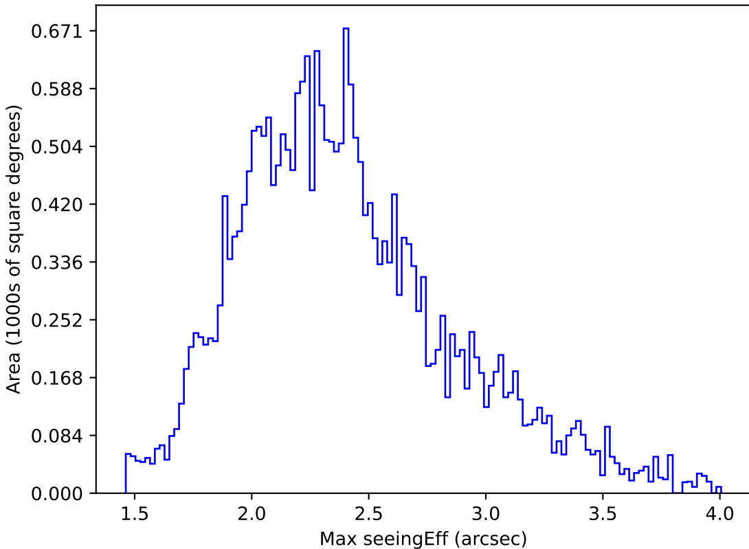
baseline_v3.3_10yrs All sky g band: Max seeingEff
